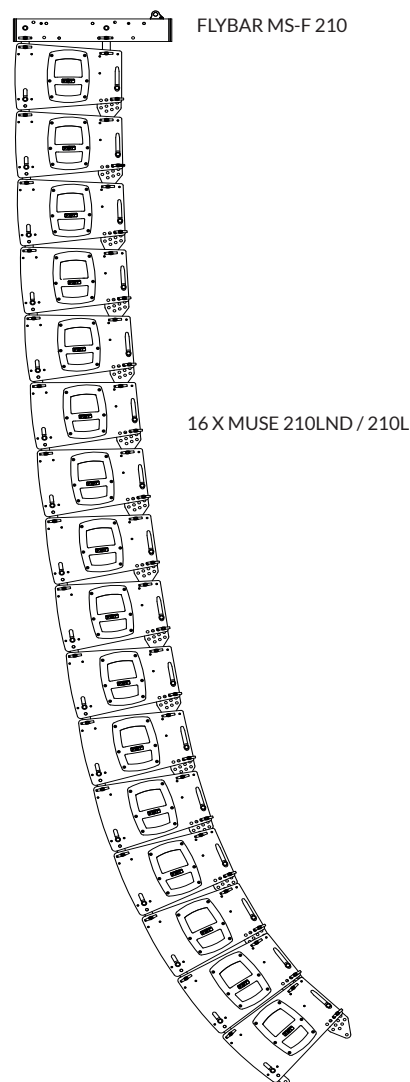
FIG.1 VERTICAL ARRAY
