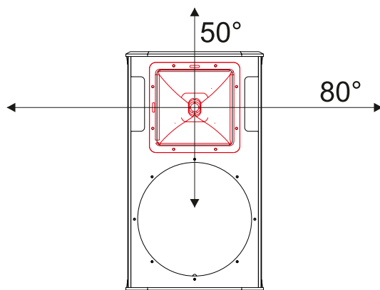
Horn coverage angle
