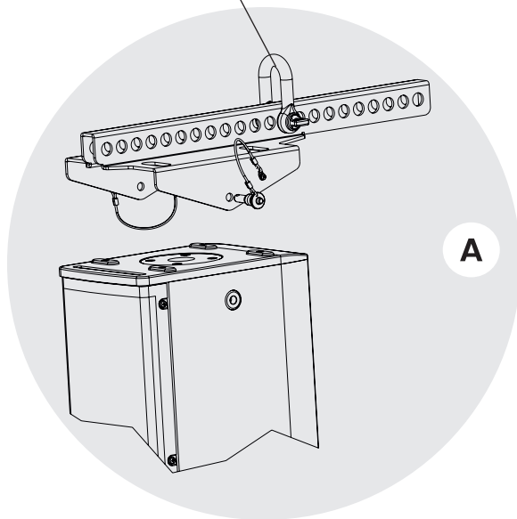
LIFTING SHACKLE
